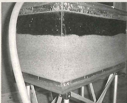
Figure 3 - False bottom flow showing uniform flow at all areas of the tun.
