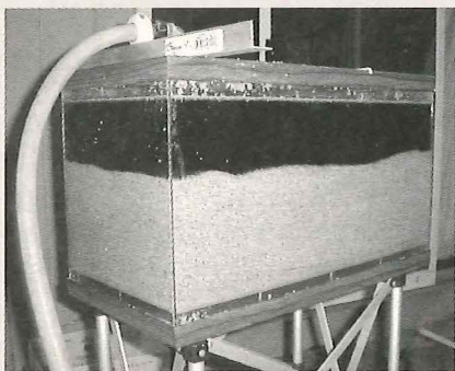
Figure 2 - Experimental setup showing dyed sparge water before flow begins.
